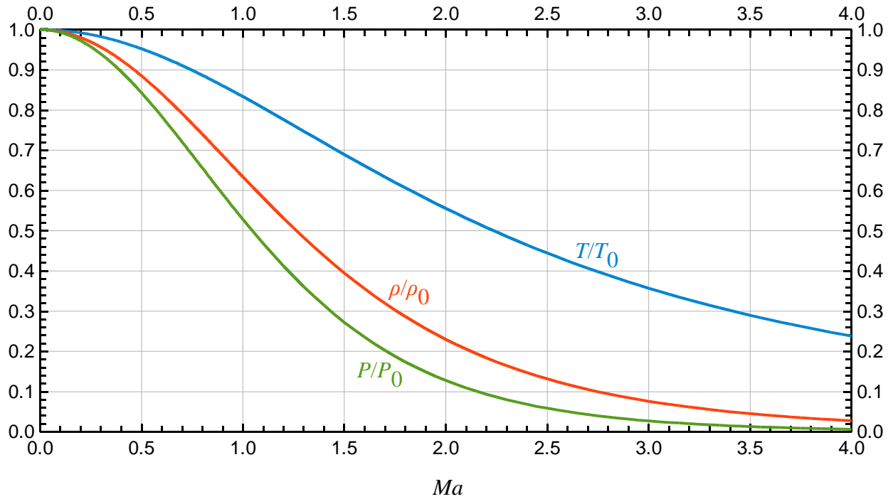
Isentropic Compressible Flow of an Ideal Gas with k=1.4 (e.g. Air)
