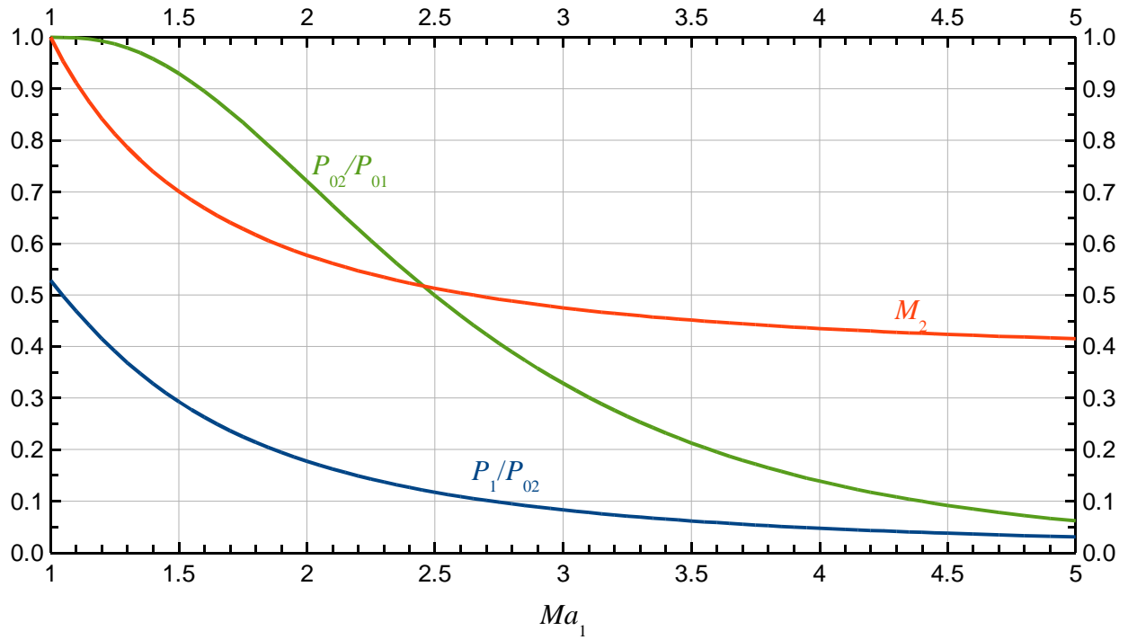
Normal Shock Factors for an Ideal Gas with k=1.4 (e.g. Air)
